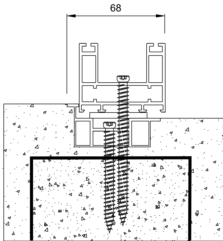
Sliding Window & Door
